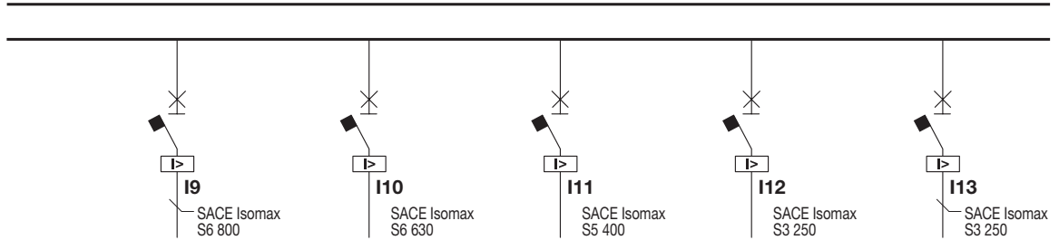
Single-line diagram
